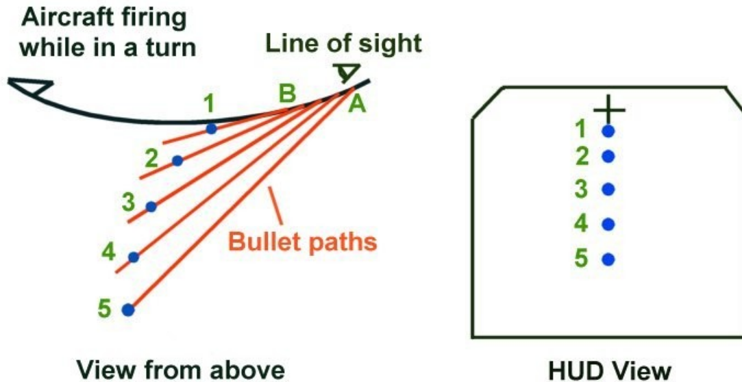
Figure 23– Projectile path
